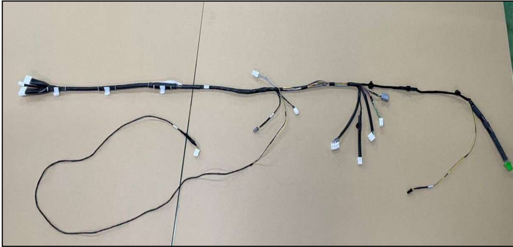
Roof Harness
