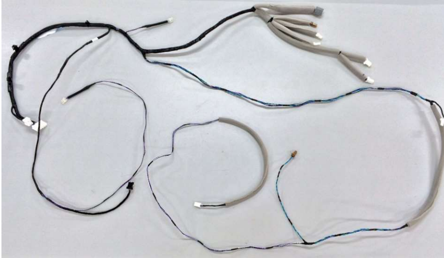
Roof Harness
