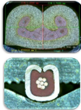
Cross section terminal machine
